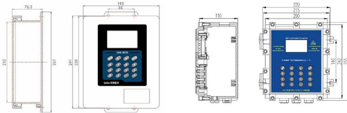
Standard Transmitter
