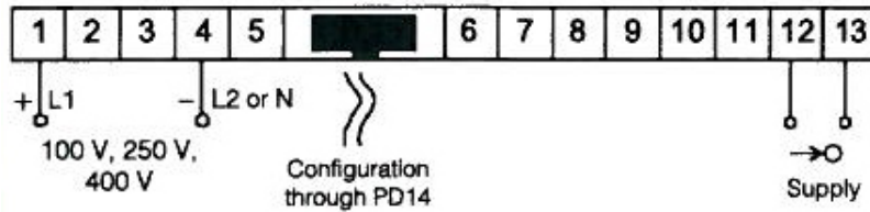
Electrical connection of the N25Z and N25H meters for voltage measurement (frequency: only N25Z )
