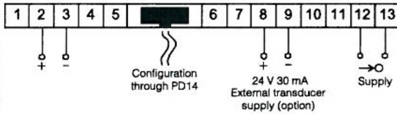
Electrical connection of the N25S meter
