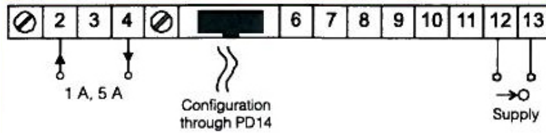
Electrical connection of the N25Z and N25H meters for current measurement
