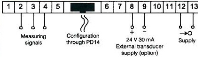
Electrical connection of the N25T meter
