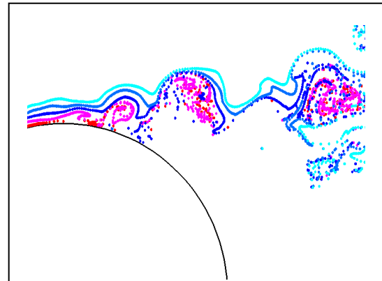
Fig. 9: Stream lines illustration at the separation area of a cylindrical shaped pitot tube sensor. Using a finite-element-method calculation, this computer graphic shows the fluid conditions at a Reynolds number Re = 20.000
