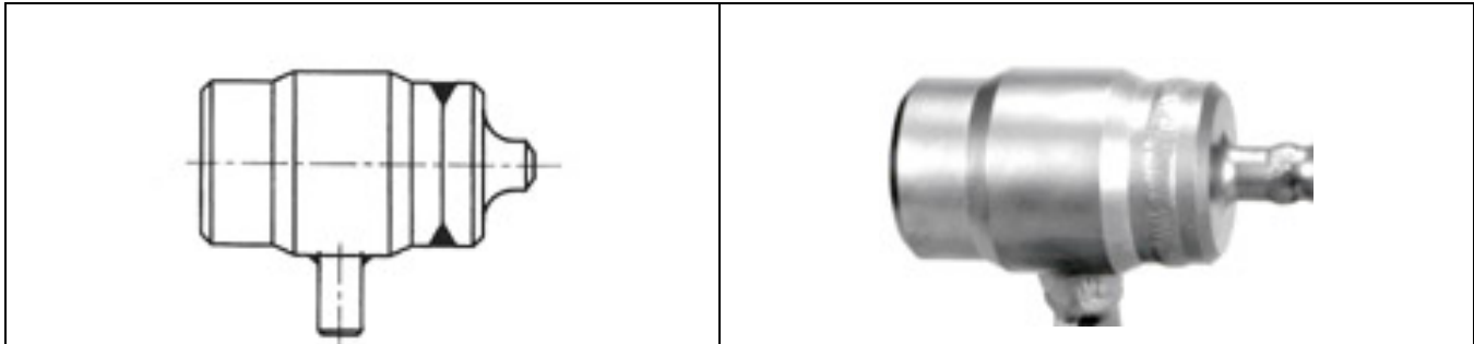
Fig 60: Condensate pots, Dimensions \varnothing 3.54 x 0.69 inches (90 x 17,5 mm) with weld sockets 0.84 inches (21,3 mm)
