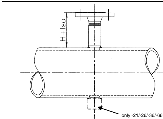
Fig. 37: Dimension H for flanged process connection
