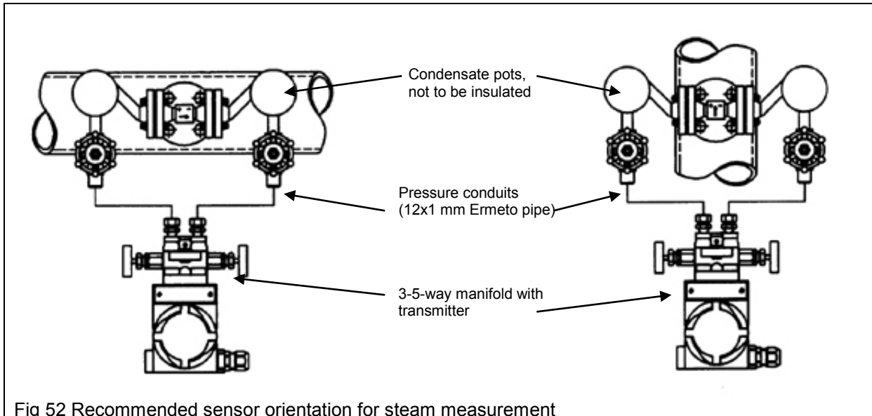
Fig 52 Recommended sensor orientation for steam measurement
