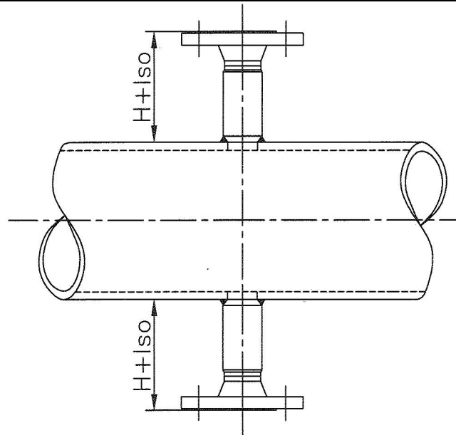
Fig. 39: Dimension H for IBF-100 (two flanges)
