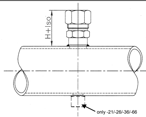
Fig. 38: Dimension H for threaded process connection
