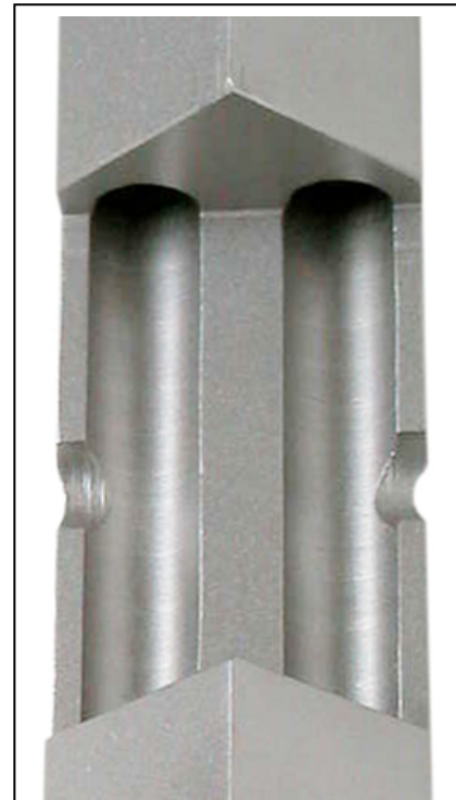
Fig. 8: Sensor profile of pitot tube model 35/36 in a cut-away view to illustrate the two pressure channels near the pressure ports..
