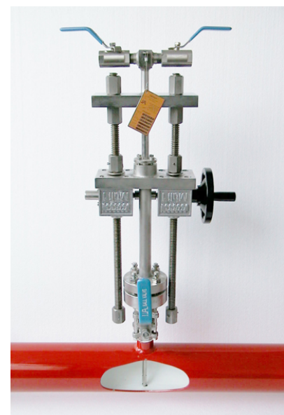
Fig 2: Flo-Tap pitot tube sensor type Itabar® FTM-20 for installation and removal under pressure
